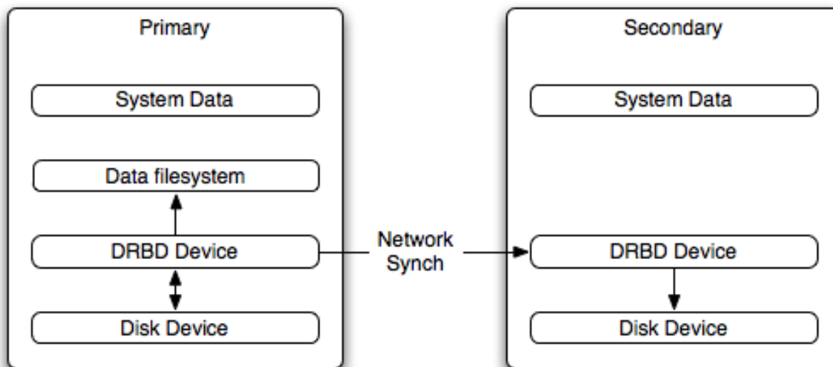
Figure 14.1. DRBD Architecture
