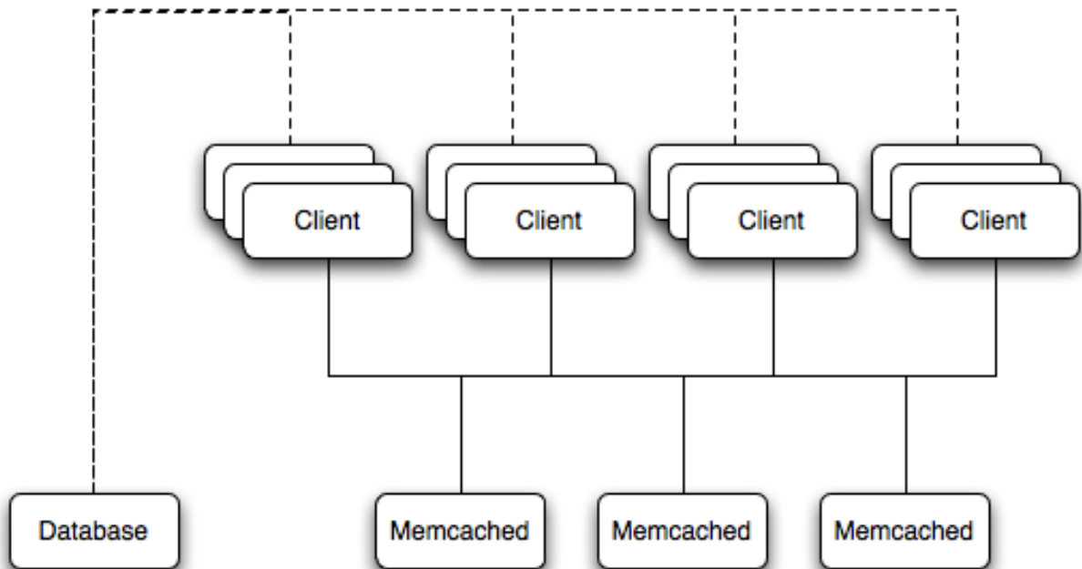
Figure 16.1. memcached overview
